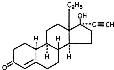
Norgestrel C_{21}H_{28}O_2 M.W. 312.45
